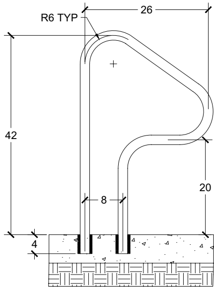
S-326 Double Post Spa Rail
