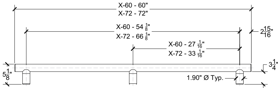
3 POST EXERCISE BARS
