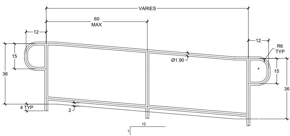
2 RAIL ADA RAMP RAIL CAN ALSO LEVEL OUT TO POST WIT NO P-LOOP
