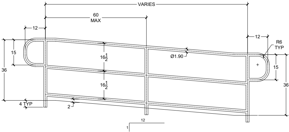
3 RAIL ADA RAMP RAIL CAN ALSO LEVEL OUT TO POST WIT NO P-LOOP
