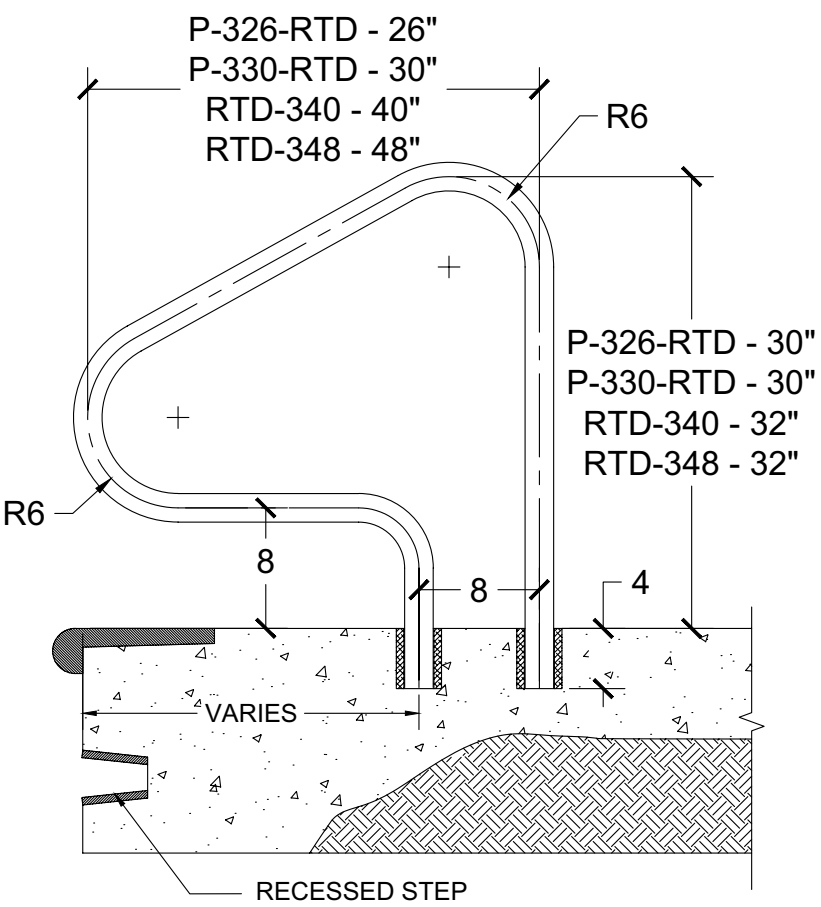
RTD POOL RAILS
